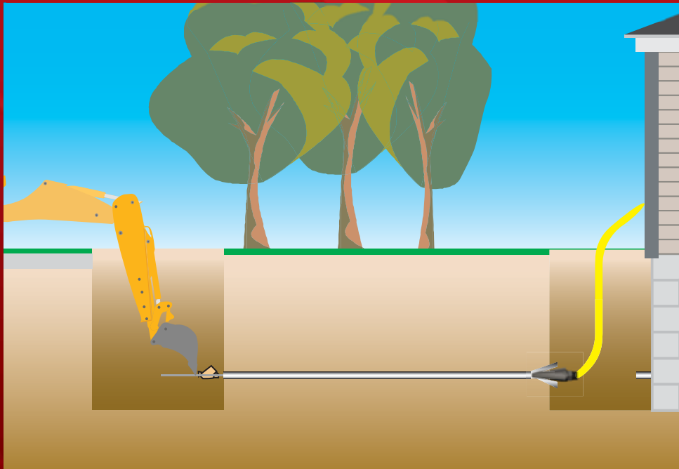
Water Line Slitter Job Site - A typical job site with the Water Line Slitter set up at the house and the backhoe setup at an exit pit. The backhoe pulls on the cable, pulling the slitter and new service pipe simultaneously.
